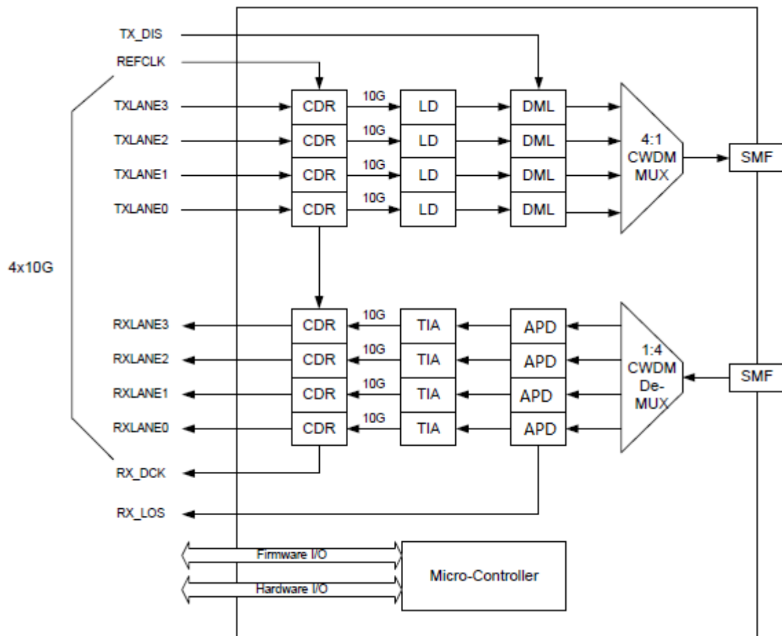
Transceiver functional diagram
