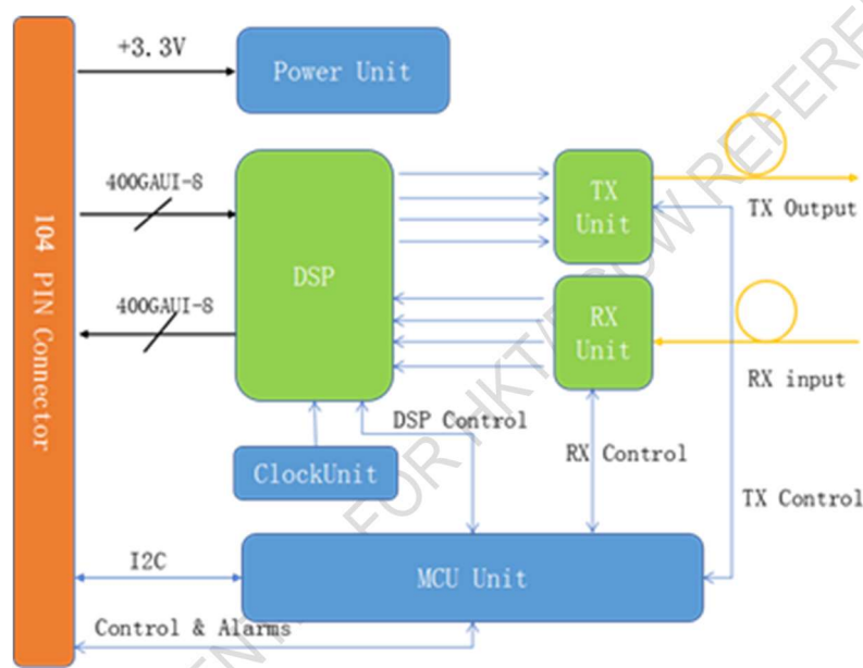
Figure 2 Module Block Diagram
