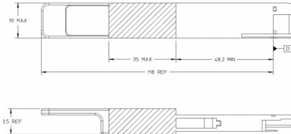
Figure 9 Dimensions
