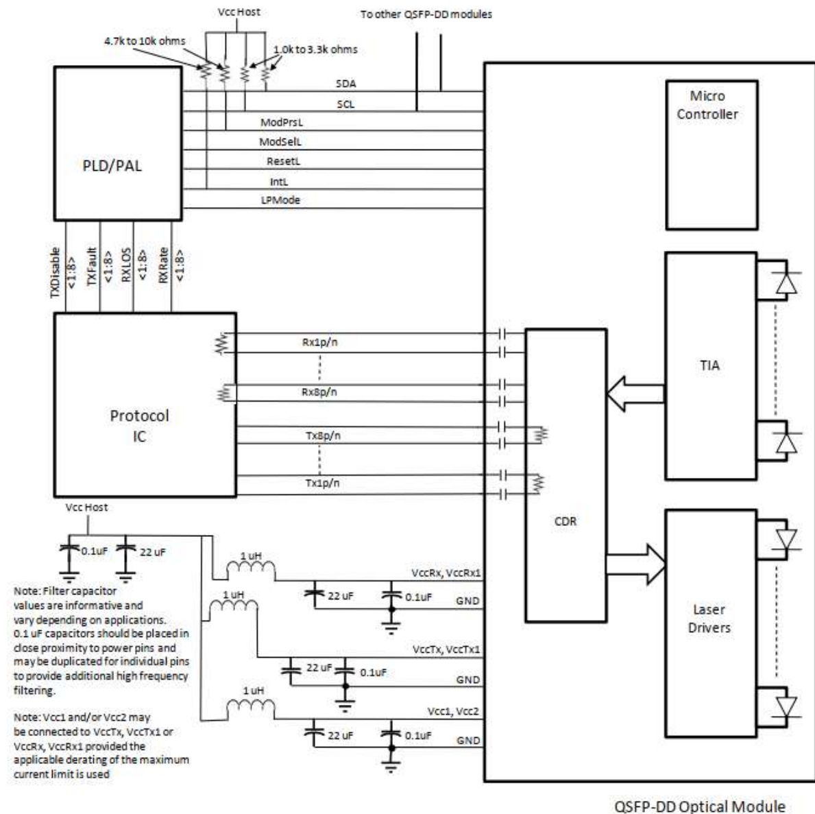
Figure 6 IIC Interface Reference Termination Mode
