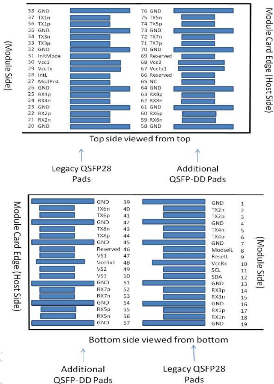
Figure 7 PIN assignment
